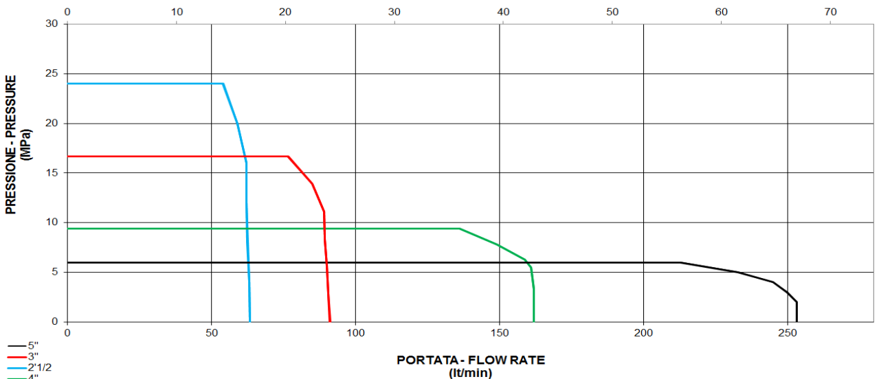
PORTATA - FLOW RATE (gpm)
