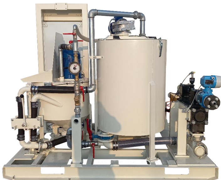
LCD Pump Control panel (optional) with recording system and preset volume / pressure injection control
