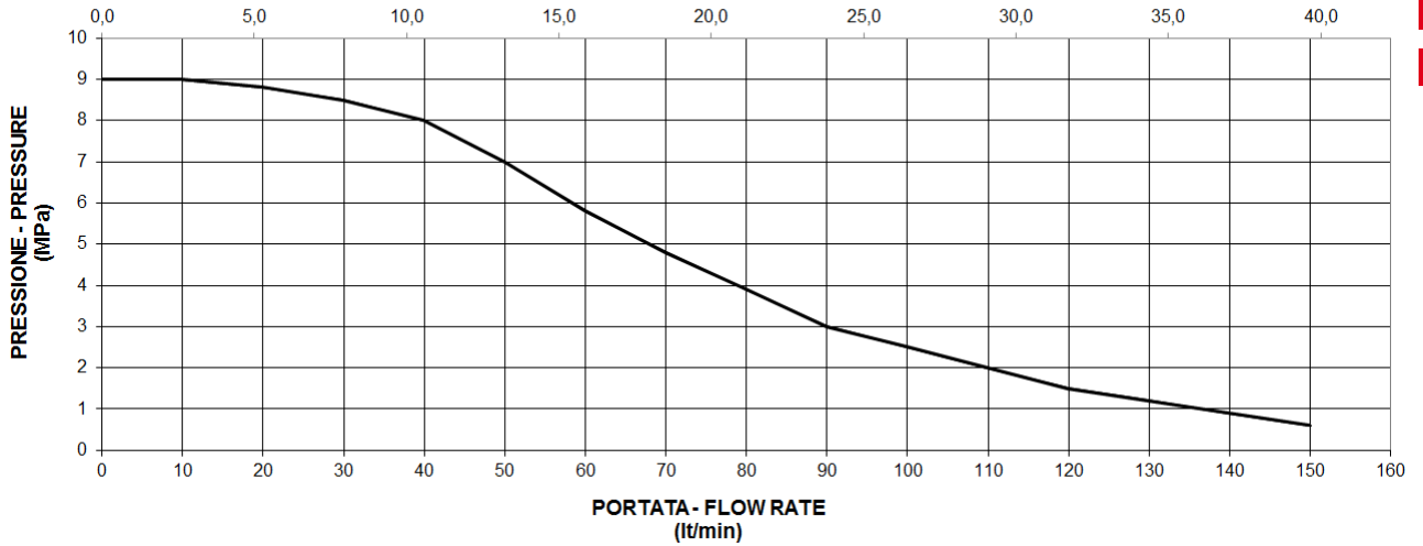
DIAGRAMMA PORTATA - PRESSIONE PRESSURE-FLOW RATE DIAGRAM
