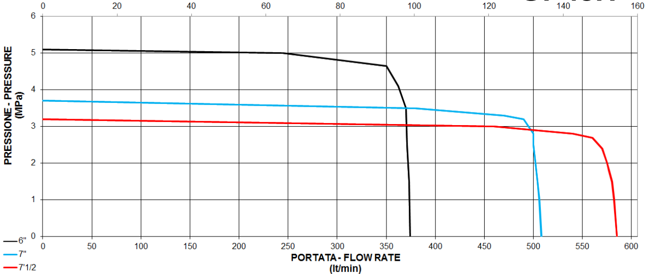
DIAGRAMMA PORTATA - PRESSIONE PRESSURE-FLOW RATE DIAGRAM
